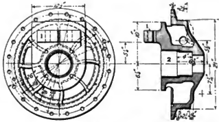
Figs. 918-919. Back Head. Cylinder Heads, Atlantic (4-4-2) Locomotive.
